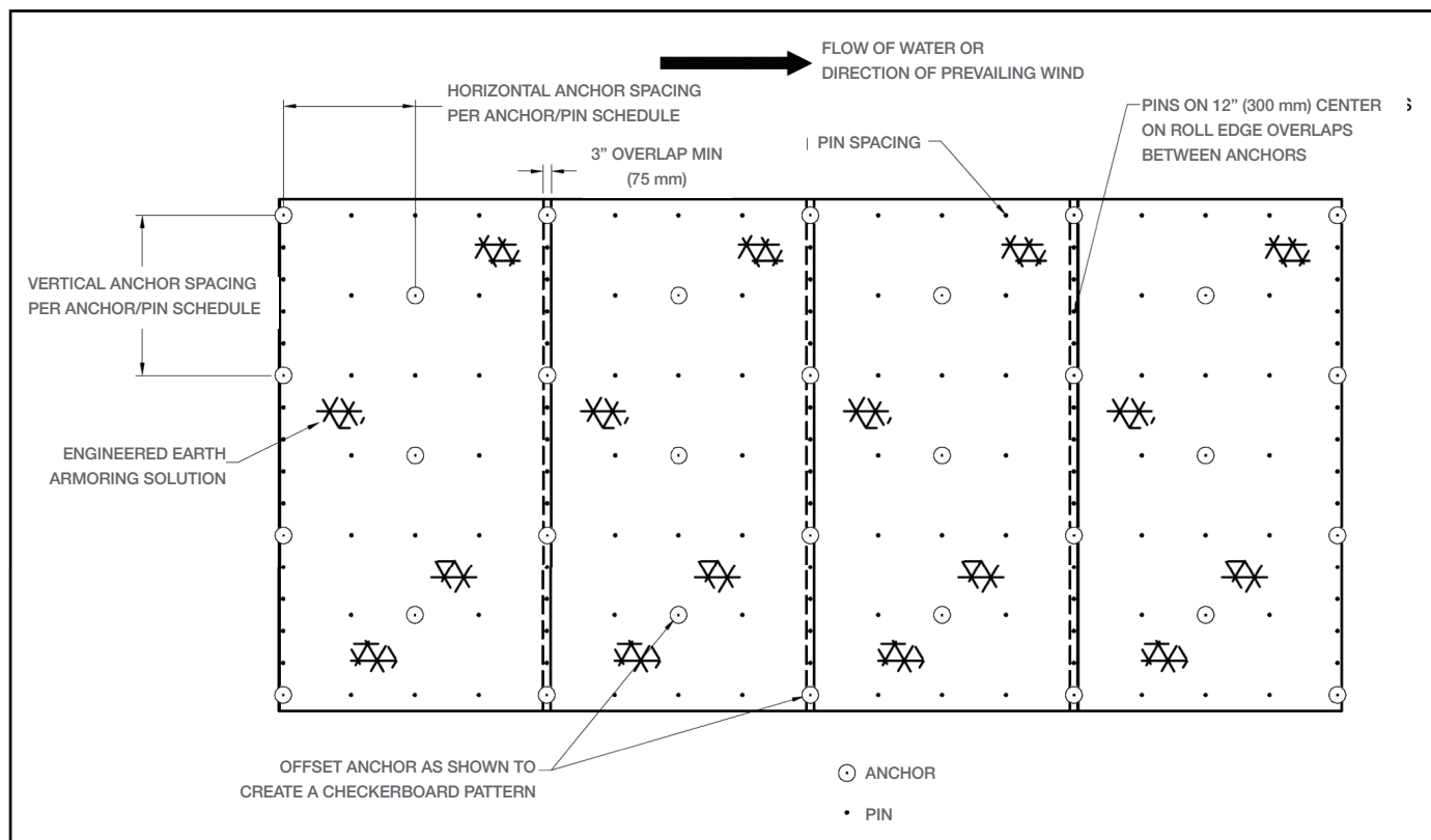
Figure 3 - Typical Anchor / Pin Pattern
