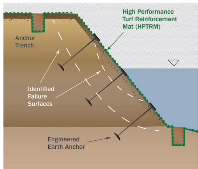
Figure 2 - Cross-Section Anchoring Past Failure Plane
